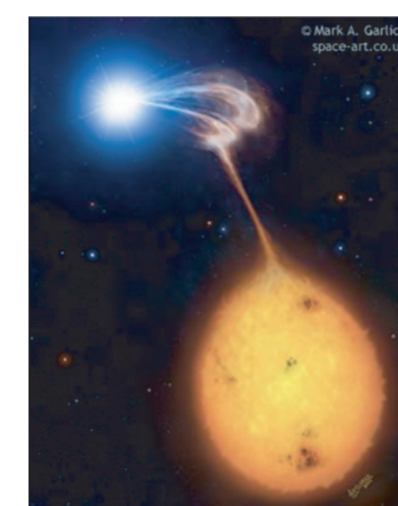
Figure 3. Artist rendition of a polar. The magnetic field of the white-dwarf totally prevents the formation of an accretion disk. Instead, the magnetic field redirects all of the incoming gas toward the magnetic poles of the white dwarf. Image permission courtesy of Mark A. Garlick.
